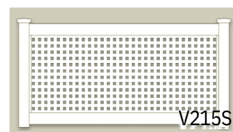
SQUARE LATTICE
